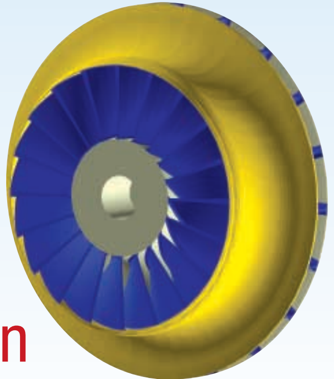
Geometry of the impeller for an expansion turbine
