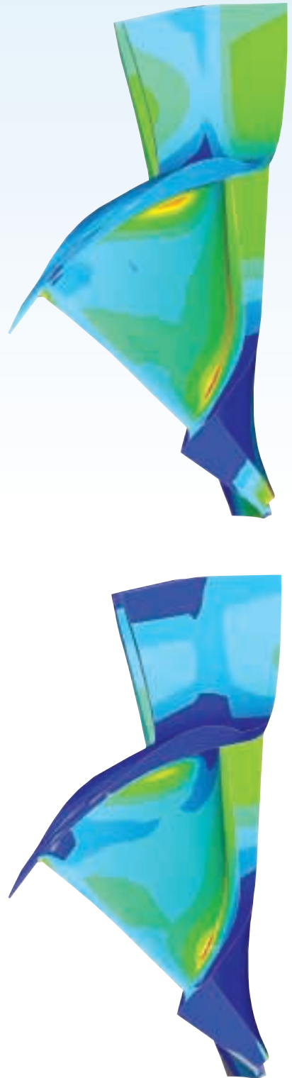
ANSYS Mechanical simulation results showing maximum principal (top) and radial (bottom) stress distributions for one impeller design. Red indicates area of high stress.
